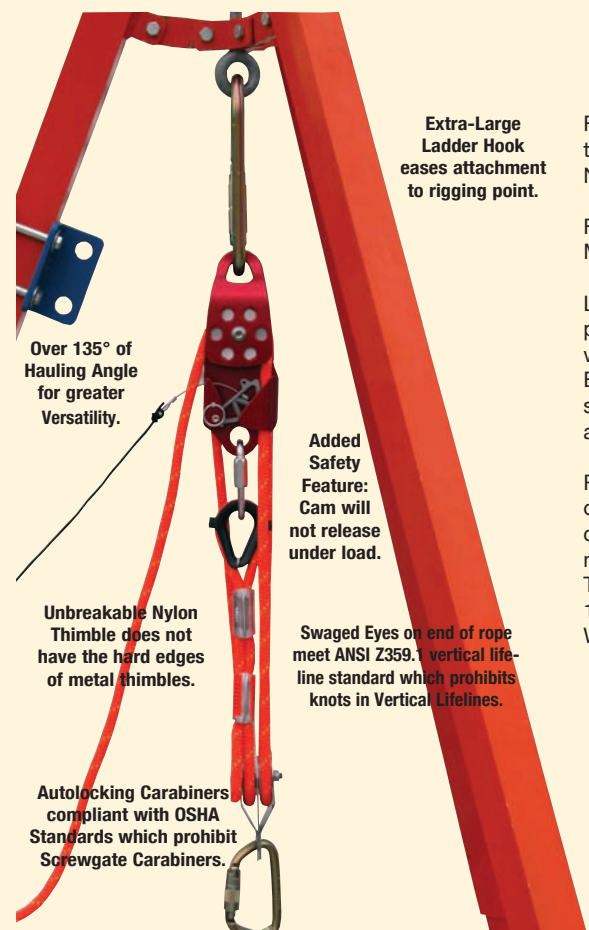
RT Extractor show with H.D. Tripod (not included with kit)
